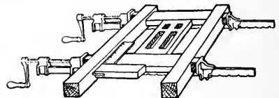
FIG. 416. TESTING FRAME FOR SQUARENESS.
